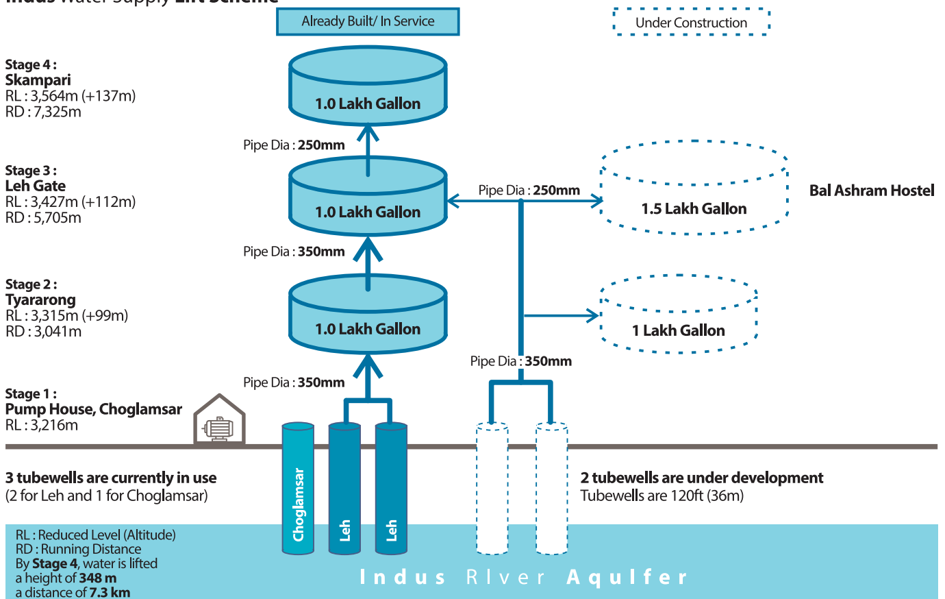
Figure 9: Indus Water Supply Lift Scheme
