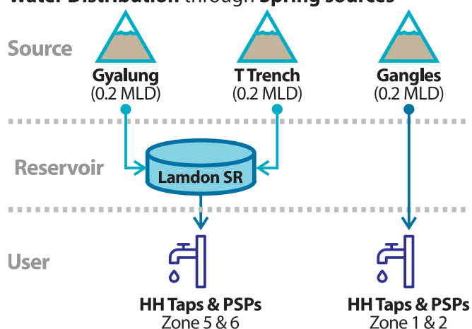
Figure 8: Schematic diagram of Water Distribution through Spring sources
