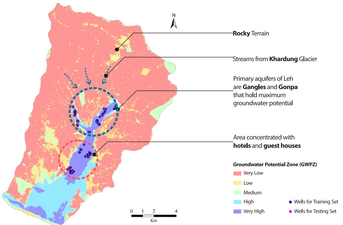
Figure 7: Groundwater Potential Zone of the Leh Valley Catchment (Balamurugan et al., 2017)
